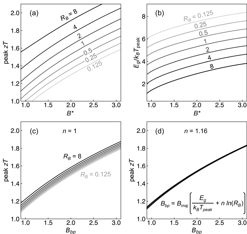
Fig. 6 (a) Peak zT and (b) E_g/k_B T_{peak} plotted against B^* (eqn (17)) for different values of R_B . Peak zT plotted against B_{bp} (eqn (18)) is shown for (c) n = 1 and (d) n = 1.16 .
