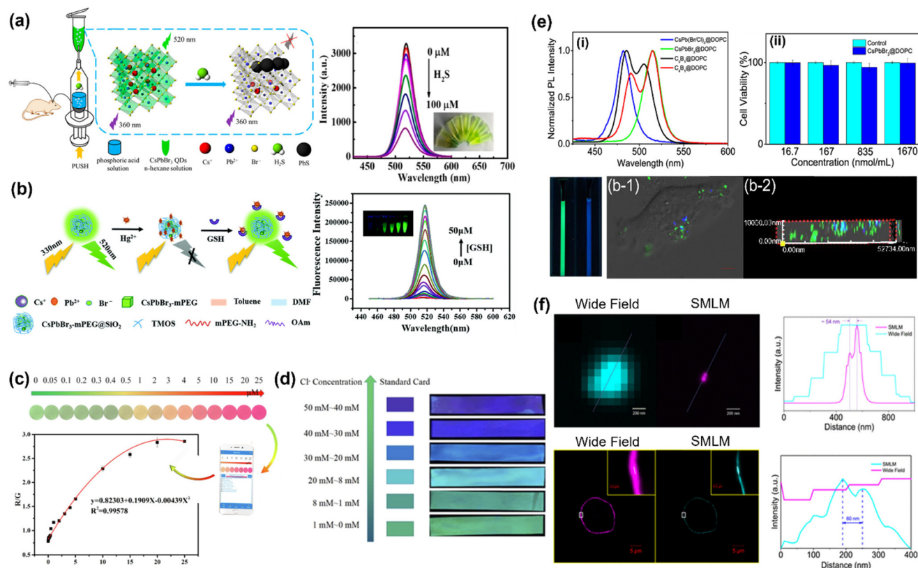
Fig. 6 (a) Schematic illustration of H 2 S detection in a rat brain microdialysis sample and FL spectra of CsPbBr 3 NCs upon the addition of different concentrations of H 2 S in the range of 0–100 \mu M. 201 (b) "On-off-on" type FL detection of Hg 2+ and glutathione (GSH) based on CsPbBr 3 -mPEG@SiO 2 NCs. 202 (c) Fast visual green-red switching sensor for tetracycline detection based on MAPbBr 3 NCs with linear response in the range of 0–25 \mu M, which can be used for detection using a smart phone software. 203 Reproduced and/or modified with permission from the listed references. (d) Colorimetric paper test strips based on CsPbBr 3 NCs for the detection of Ciprofloxacin solution in a range from 0 to 50 mM and under UV light (365 nm). 204 (e) PL emissions from CsPbCl 3 and CsPbBr 3 coated with DOPC/DOTAP and DSPE-mPEG-FA, their corresponding in vitro viabilities in HeLa cells, and fluorescence confocal microscopy images showing internalization in HeLa cells and multiplexed luminescence capabilities. 147 (f) Fluorescence microscopy (left) and super-resolution microscopy (right) imaging of nuclear lamina (top) and exosomes (bottom) using CsPb(Cl 1-x Br x ) 3 HPNCs, and the corresponding FWHM of each signal. 189 Panel 6a adapted with permission from ref. 240 Copyright 2019 American Chemical Society.
