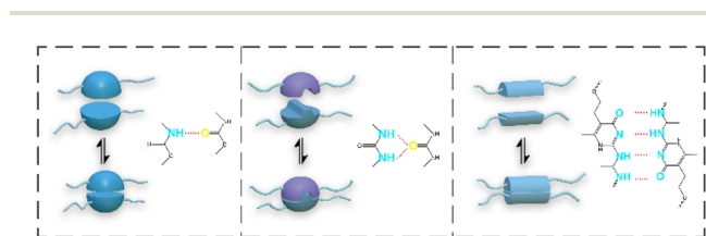
Fig. 2 The three typical hydrogen bonds in PU.
