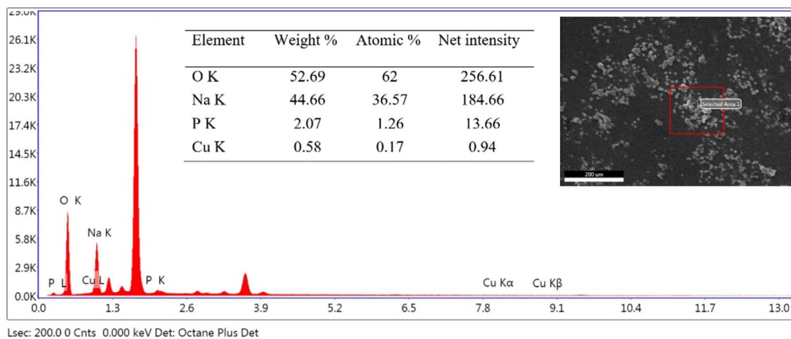
Fig. 2 A typical EDS spectrum of \text{NaLi}_2\text{PO}_4:\text{Cu}(\text{II}) (0.1 mol%) material. The SEM image and the elemental composition are also shown in the inset.
