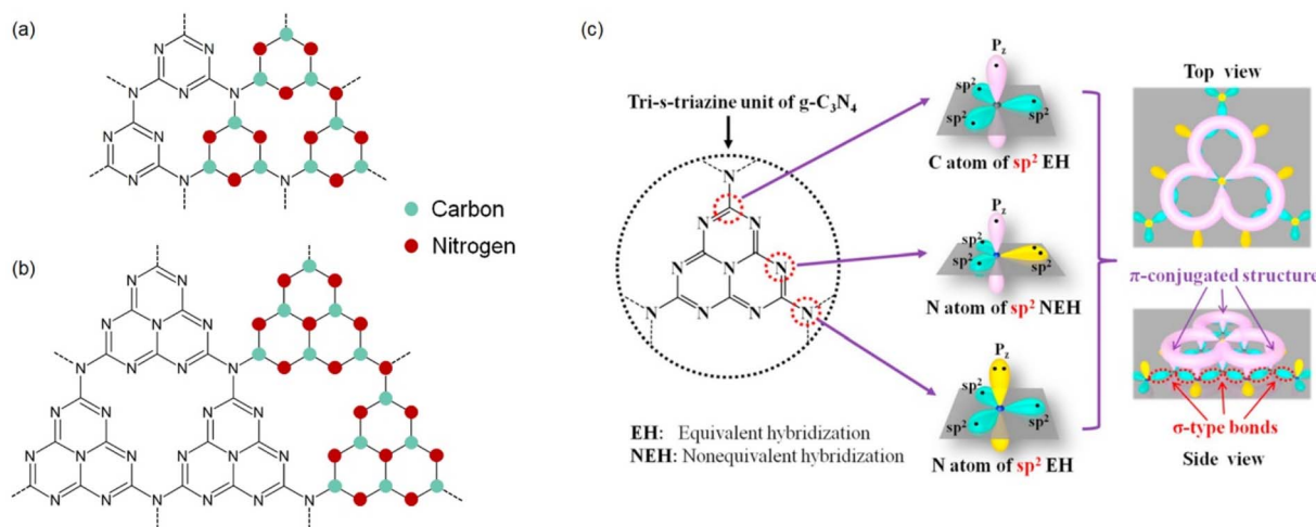
Fig. 1 Schematic illustration of chemical structure of g-C_3N_4 : (a) triazine structure and (b) tri-s-triazine structure. (c) Hybrid structure and \pi -conjugated structure of the tri-s-triazine unit of g-C_3N_4 . Reproduced from ref. 23 with permission. Copyright 2019, Elsevier.
