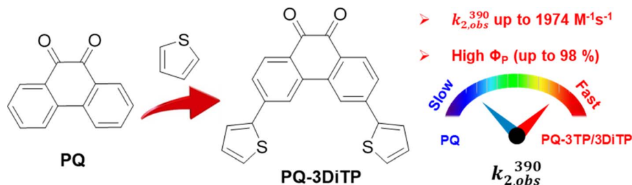
Scheme 1 Comparison of photocycloaddition of 9,10-phenanthrenequinone ( PQ ) with electron-rich alkenes ( ERAs ). k_{2,\text{obs}}(390) observed second-order reaction rate; and \Phi_p : photoreaction quantum yield.
