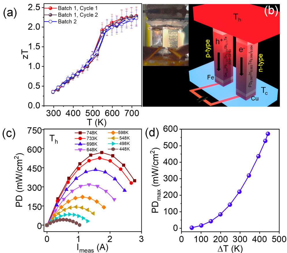
Fig. 6 (a) zT of BM + SPS processed \text{Ge}_{0.84}\text{Pb}_{0.025}\text{Sn}_{0.025}\text{Sb}_{0.11}\text{Te} is reversible over the temperature cycle and batch, (b) schematic representation of the double leg device where the \text{Ge}_{0.84}\text{Pb}_{0.025}\text{Sn}_{0.025}\text{Sb}_{0.11}\text{Te} (BM + SPS) sample is used as the p-type leg and \text{Pb}_{0.997}\text{In}_{0.003}\text{Te}_{0.996}\text{I}_{0.004} is used as the n-type leg (inset shows the original device photograph), (c) output power density (PD) as a function of measured current at different temperature gradients and (d) maximum output power density ( \text{PD}_{\text{max}} ) as a function of temperature gradient of the double leg TE device.
