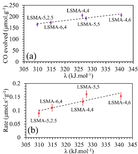
Fig. 10 Amounts of \text{CO} evolved (a) and re-oxidation rates (b) as a function of overall bond energies for \text{La}_x\text{Sr}_{1-x}\text{Mn}_y\text{Al}_{1-y}\text{O}_3 oxygen carriers.
