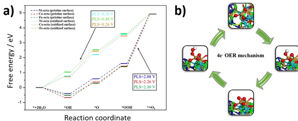
Fig. 6 (a) Quantum-theoretical calculations at the level of density functional theory (DFT) on the electrocatalytic OER performance in FCNSSLi, and (b) the computational optimized OER intermediates on Fe in FCNSSLi.
