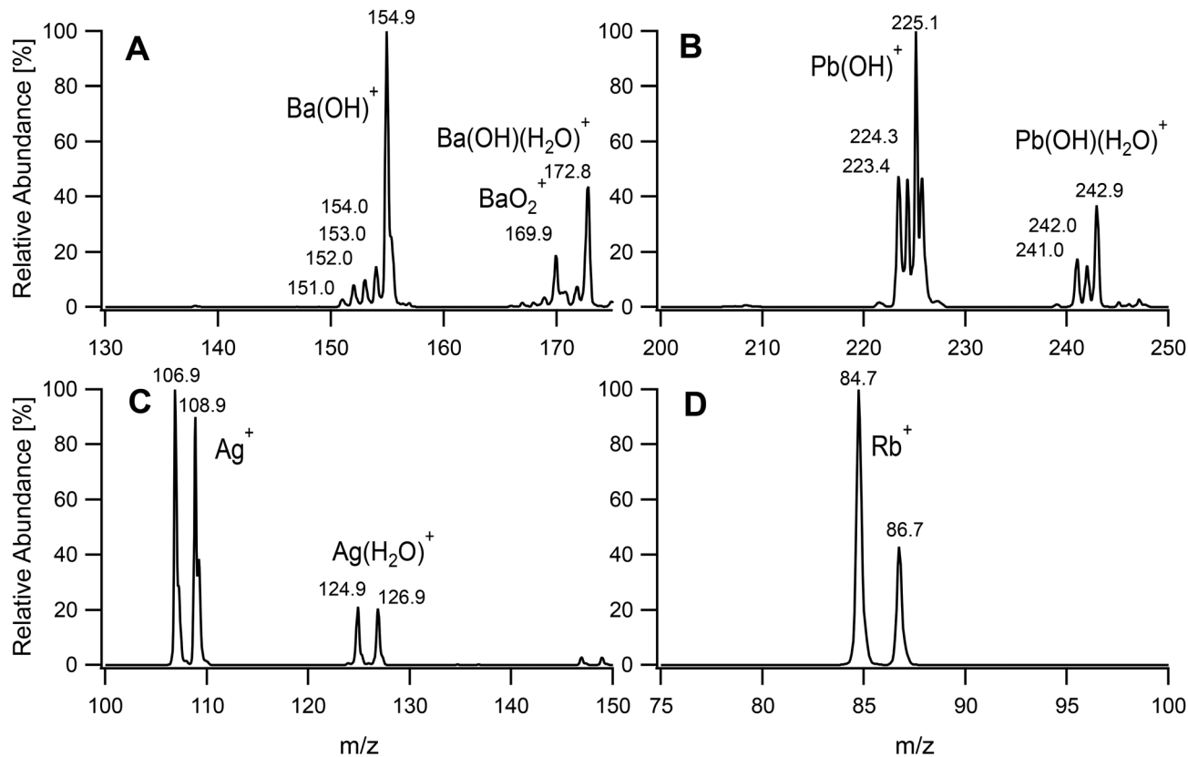
Fig. 5 Mass spectra of selected metal salt solutions at 50 μM. BaCl 2 (A), Pb(NO 3 ) 2 (B), AgNO 3 (C) and RbCl (D).
