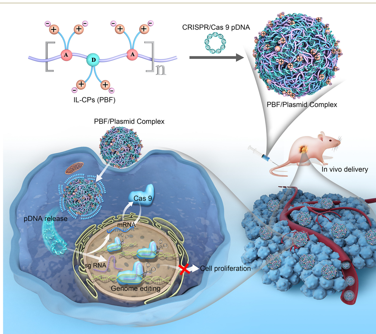
Scheme 1 Schematic illustration of IL-CPs-mediated delivery of the CRISPR-Cas9 plasmid and gene therapy for tumor.
