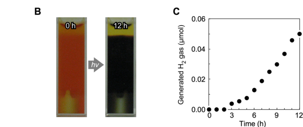
Fig. 8 (A) Photoinduced H 2 -generating system composed of a poly(NIPAAm- co -Ru(bpy) 3 - co -viologen) gel containing Pt NPs. (B) Images of the gel suspension before and after light irradiation. (C) H 2 -generation in the gel system. Reproduced from ref. 68 with permission from the Royal Society of Chemistry. Copyright 2009.
