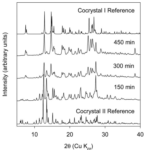
Fig. 4 XRPD data of rBN/BQ at a 1 : 2 mole ratio subjected to RAM shown in comparison to the reference powder data calculated from the published crystal structures of cocystals I and II. 440 mg of total solids and 1320 mg of zirconia beads were used for the experiment. RAM was done at 75g for all samples.
