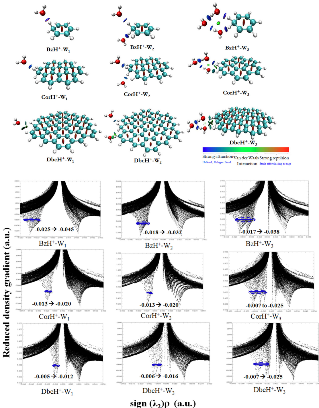
Fig. 3 Top: NCI indexes of the BzH^+-W_n , CorH^+-W_n and DbcH^+-W_n ( n = 1-3 ) clusters with an isosurface of 0.59 a.u. We show the strong and weak interaction regions in blue and green, respectively. Bottom: Bi-dimensional plots of reduced density gradient RDG versus sign(\lambda_2)*\rho of BzH^+-W_n , CorH^+-W_n and DbcH^+-W_n ( n = 1-3 ) clusters.
