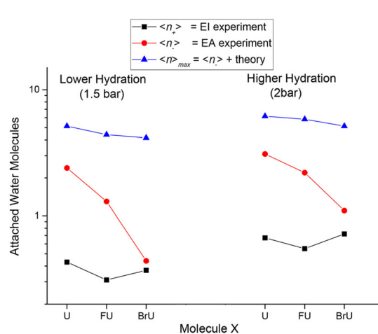
Fig. 4 The image from the work of Pořtůlka et al. showing that theory predicted increase in the energy transfer to solvent due to the electron affinity of the microhydrated halo uracils can reproduce well the fragmentation of their TNIs. For uracil (U), bromouracil (BrU) and fluorouracil (FU) shown on the x-axis the y-axis shows the detected mean size of ionic clusters upon electron attachment (red) and electron ionization (black). The blue points are mean values of neutral cluster sizes estimated based on electron affinities and under the assumption that all energy transferred to solvent leads to the evaporation of water molecules from the cluster. Reproduced from ref. 52 with permission from American Chemical Society, copyright 2017.
