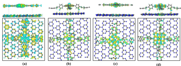
Fig. 12 Charge density difference of (a) Pc-PBBA COF Fe @C 3 N 4 , (b) COF-366 Fe @C 3 N 4 , (c) Pc-PBBA COF Co @C 3 N 4 , and (d) COF-366 Co @C 3 N 4 . The yellow and cyan colors represent electron accumulation and depletion regions, respectively. The isosurface level is set to 0.004 e Bohr -3 .
