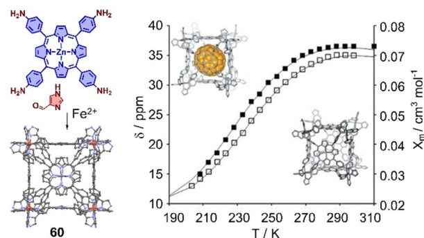
Fig. 21 Self-assembly of an octanuclear metallogage 60 and chemical shift of selected protons in temperature-dependent ^1H NMR experiments in CD_3OD . Black lines represent the calculated molar susceptibility \chi_m based on the ideal solution model. Adapted from ref. 333 with permission from Wiley-VCH, copyright 2017.
