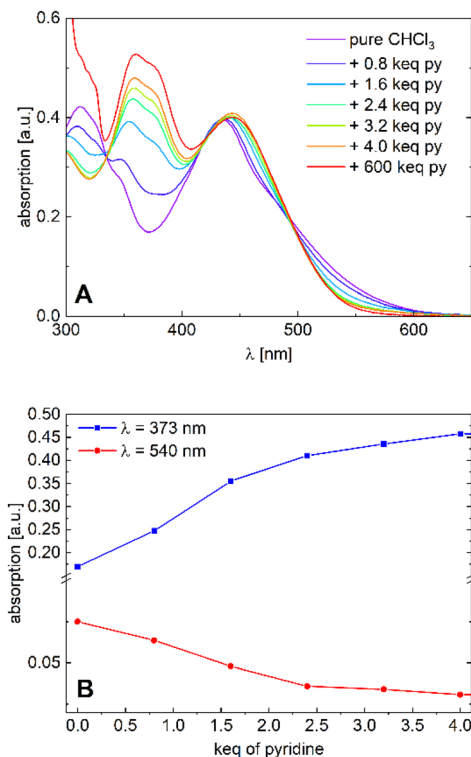
Fig. 5 (A) Absorption spectra of [\text{Ni}_2\text{L}] in varying chloroform/pyridine ratios ( c = 1.0 \times 10^{-5} M) and (B) absorption plots at \lambda = 373 nm and \lambda = 540 nm.
