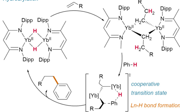
Fig. 13 Hydroarylation catalysed by an ytterbium(II) hydride complex contrasts with classical sigma bond metathesis reactivity observed for Sm(III).
