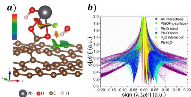
Fig. 6 a) NCI isosurface with s = 0.05 a.u. and b) s[\rho(r)] vs. \text{sign}(\lambda_2)\rho(r) graph for the adsorption Pb(OH)_2 on the GO surface.
