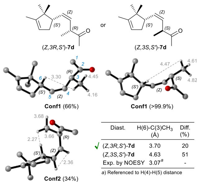
Fig. 4 DFT computed H(6)–C(3) \text{CH}_3 interproton distances ( \text{Å} ) of most stable conformers of C(3) epimers, compared to the experimental distance determined by quantitative NOE, for clarity some hydrogen atoms are omitted. In round brackets is reported the Boltzman conformer population.
