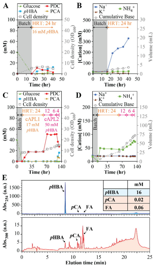
Fig. 5 MBR performance with APL and extracted APL (eAPL), with NH 4 OH used as the base for pH control. For each experiment, the gray-colored boxes indicate an initial batch period with SMB containing 40 mM glucose. Panels A and C show effluent concentrations of p HBA, PCA, PDC, and glucose, and cell density throughout the operational period. Panels B and D show effluent concentrations of Na + , K + , and NH 4 + , and the cumulative volume of base added throughout bioreactor operation. Panels A and B show data with poplar APL amended with 20 mM glucose at an HRT of 24 h. Panel C and D show MBR performance data with extracted APL media (eAPL1 and eAPL2) supplemented with 50 mM glucose, and decreasing HRTs of 24, 12, 6, and 4 h. Panel E shows HPLC chromatograms of the poplar APL at two different wavelengths, showing small concentrations of p -coumaric acid ( p CA), ferulic acid (FA), and other unidentified compounds.
