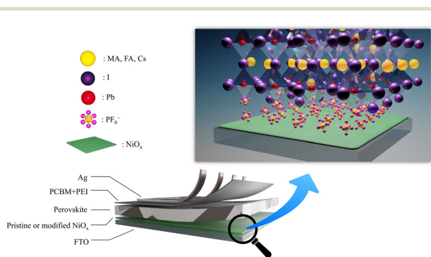
Fig. 1 Device architecture of PSCs with the enlarged illustration of the salt-modified \text{NiO}_x /perovskite interface.
