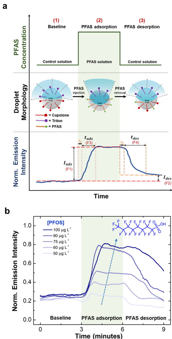
Fig. 3 (a) Graphical representation of real-time emission response of PFAS generated by applying three-step square wave input flow. Shaded area signifies the injection of PFAS solutions from t = 3 min to t = 6 min. (b) Real-time emission responses to different concentrations of PFOS in Milli-Q water. Each response is an averaged response from separate experiments ( N \geq 5 ).
