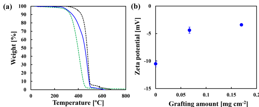
Fig. 2 (a) Thermogravimetric curves of the unmodified polyethylene substrate (black, dashed), PMEAs (green, dashed) and grafted membrane (blue, solid). (b) Relationship between the grafting amount and the zeta potential of the membrane surface.
