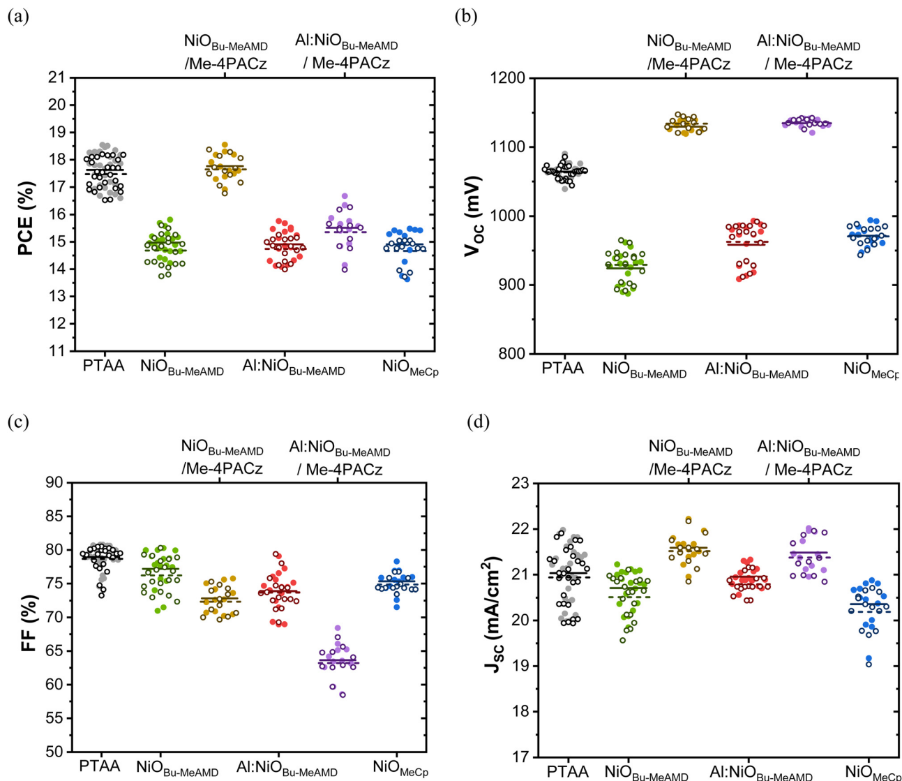
Fig. 1 PV parameters of the different HTL-based devices (a) PCE, (b) V_{OC} , (c) FF, and (d) J_{SC} . The filled circles and the solid line represent the reverse J - V scan whereas the empty circles and the dashed line represent the forward J - V scan. The solid and dashed lines represent the mean value of the PV parameter during the reverse and forward scans respectively. These data are collected from several batches on 30 devices with PTAA, 20 devices with NiO and 15 devices with NiO/SAM.
