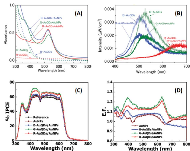
Fig. 22 (A) UV-visible absorption spectra and (B) fluorescence spectra of AuQDs and AuQD: AuNP aqueous solution; (C) %IPCE and (D) E. F. profiles for OSCs incorporating AuQDs and plasmonic AuNPs. Reproduced from ref. 37 with permission from the Royal Society of Chemistry (CC BY-NC 4.0).
