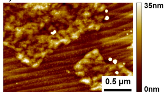
Fig. 4 AFM topography of (a) pristine CVD-G/Cu and (b) functionalized CVD-G/Cu. The functionalized CVD-G/Cu presents both metallic Cu (horizontal lines) and oxidized regions.
