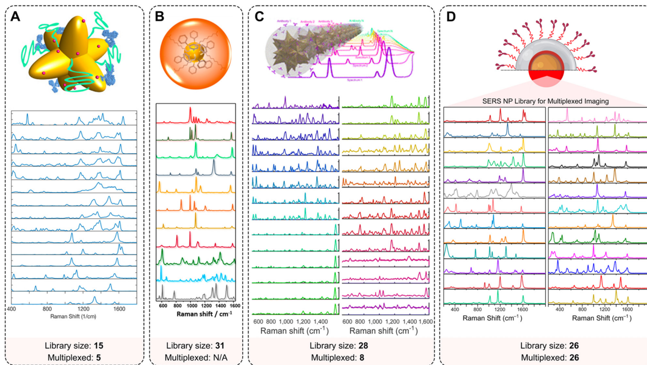
Fig. 7 Multiplexing capabilities of SERS NPs. Examples of extended spectral libraries of SERS NPs: (A) SERS spectra of the 15 selected Raman reporters on gold nanostars (adopted with permission from ref. 170. Copyright Authors); (B) SERS spectra of 11 representative SERS-encoded NP colloids from a 31-membered panel (adopted with permission from ref. 93. Copyright 2015 American Chemical Society); (C) uniquely identifiable spectra, shown here after baseline subtraction and averaging for a 28-membered SERS NP panel (adopted with permission from ref. 98. Copyright Authors); (D) Raman signatures from a 26-membered library of SERS NPs (adopted with permission from ref. 94. Copyright 2022 American Chemical Society).
