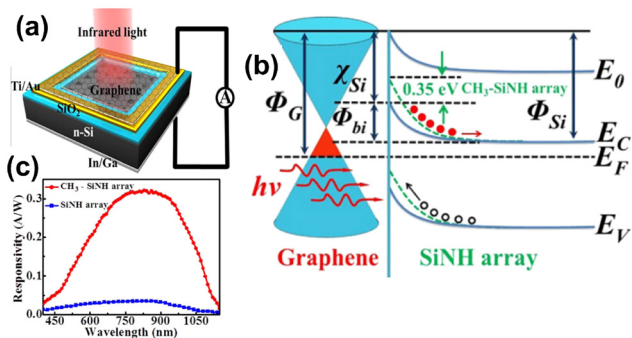
Fig. 14 (a) Schematic of a graphene/Si nanohole array Schottky junction based self-powered near-infrared photodetector, (b) energy band diagram of the device with and without surface passivation under light, and (c) responsivity with and without surface passivation for different wavelengths. 112 Published with "Optica Publishing Group" as open access, 2015.
