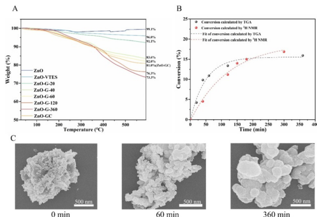
Fig. 2 (A) TGA of ZnO, ZnO-VTES, ZnO-GC and ZnO-G with different polymerization times. (B) Conversion vs. time for the polymerization of MAGH and MAG determined by TGA and ^1\text{H} NMR. (C) SEM images of ZnO-G with polymerization times of 0, 60 and 360 min.
