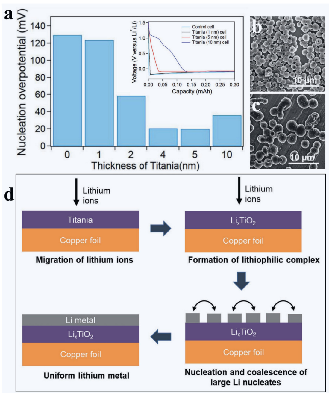
Fig. 11 Effects of ALD \text{TiO}_2 on the surface lithiophilicity of the Cu foil. 158 (a) First cycle nucleation overpotential as a function of ALD \text{TiO}_2 thickness (inset: voltage profiles for the first cycle of lithium plating for control cell, 1, 5, and 10 nm \text{TiO}_2 cells). Top-view SEM images of 0.3 \text{ mA h cm}^{-2} lithium embryos formed in (b) the control cell and (c) 5 nm \text{TiO}_2 cell. (d) Schematic illustration of the role of \text{TiO}_2 as a nucleation layer for electrodeposited Li. The electrolyte is 1 M LiTFSI in 1/1 volume ratio of DOL/DME with 1 wt% \text{LiNO}_3 . Reprinted (adapted) with permission from ref. 158. Copyright (2020) John Wiley and Sons.
