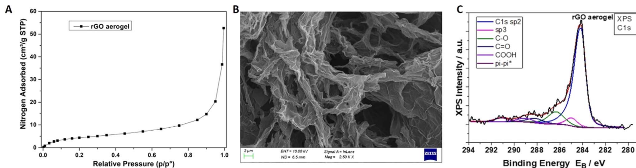
Fig. 4 (A) Nitrogen adsorption isotherm, (B) SEM image and (C) deconvoluted C 1s XPS spectrum of a neat rGO aerogel.
