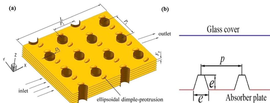
Fig. 16 Protrusion used in HX. (a) Ellipsoidal dimple. 180 (b) Frustum-shaped. Reproduced with permission 178 copyright © 2023 International Solar Energy Society.
