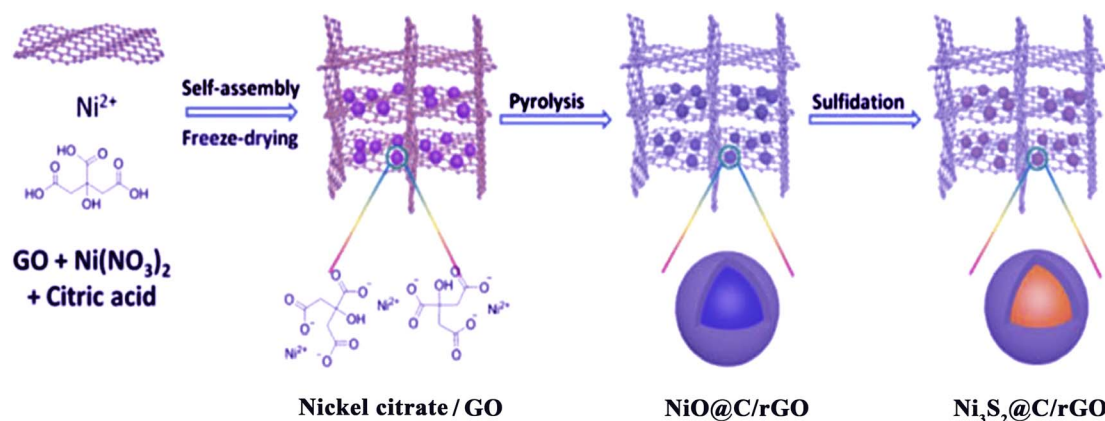
Fig. 4 Schematic of the synthesis of dual carbon-modified Ni 3 S 2 -C/rGO. 152
