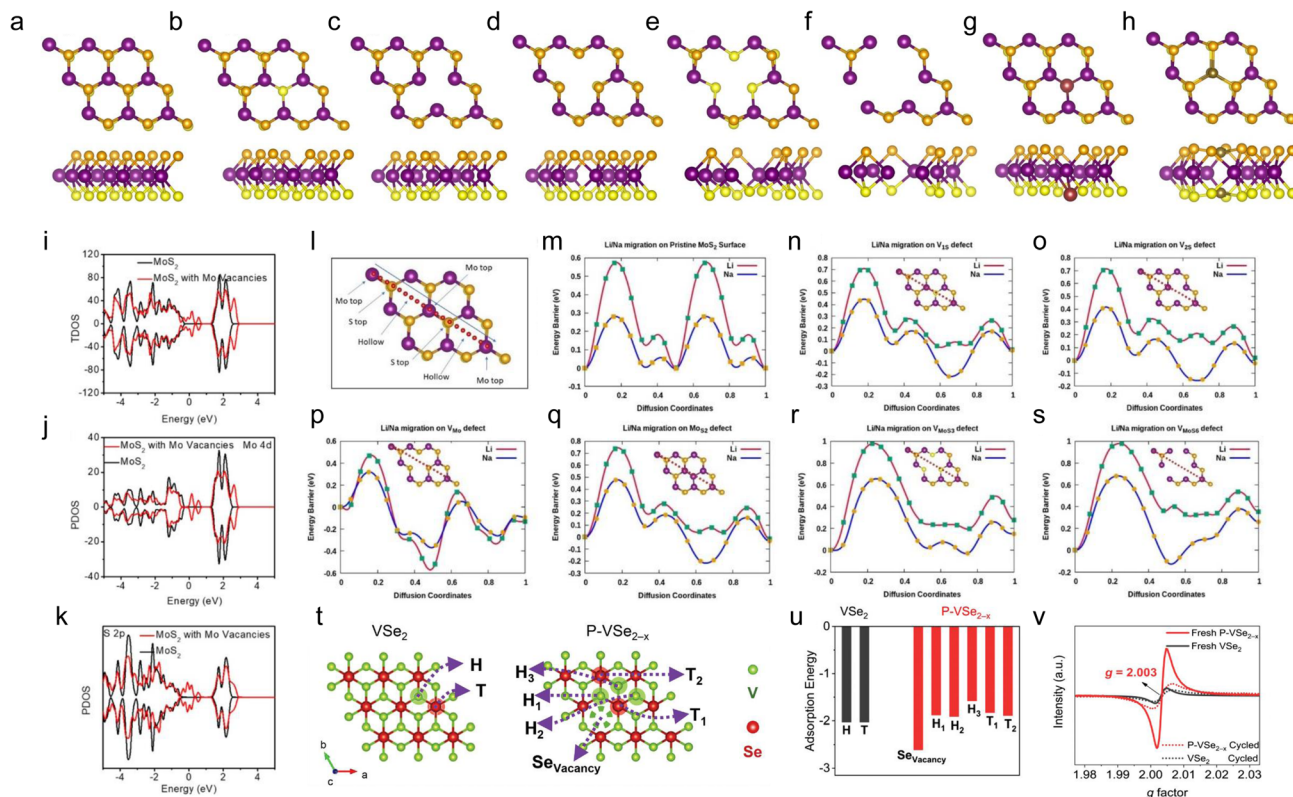
Fig. 3 Optimized geometry of various defects in monolayer MoS 2 . (a) Pristine MoS 2 , (b) V 1S , (c) V 2S , (d) V Mo , (e) V MoS3 , (f) V MoS6 , (g) MoS 2 , and (h) S 2Mo2 vacancies. The purple and yellow colored balls denote Mo and S atoms, respectively. The top layer of S atoms is in golden yellow color, and the bottom layers are in light yellow color. In the MoS 2 vacancy, the maroon-colored ball represents the antisite Mo substituting a sulfur atom. In the S 2Mo vacancy, the gray ball represents the antisite S substituting a Mo atom. The diffusion path for Li/Na on MoS 2 with defects. Total (i) and partial (j and k) charge density of states of MoS 2 with Mo vacancies and pristine MoS 2 . Diffusion energy profiles for Li/Na diffusion barriers for (l) pristine MoS 2 , (m) Li/Na migration path on pristine MoS 2 , (n) monosulfur vacancy, (o) disulfur vacancy, (p) Mo vacancy, (q) MoS 2 vacancy, (r) MoS 3 vacancy, and (s) MoS 6 vacancy. (t) K + adsorption sites on VSe 2 and P-VSe 2-x , and (u) their corresponding adsorption energies. (v) EPR spectra of VSe 2 and P-VSe 2-x electrodes before and after one galvanostatic charge–discharge cycle. Reproduced with permission from (a–h and l–s) ref. 124. Copyright 2019, American Chemical Society; (i–k) ref. 126. Copyright 2019, American Chemical Society; (t–v) ref. 42. Copyright 2023, Wiley-VCH.
