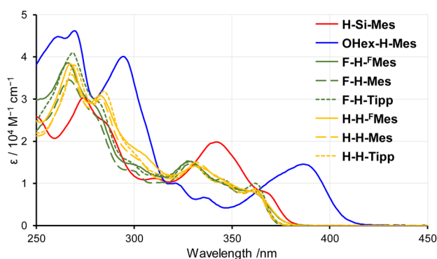
Fig. 2 UV-vis absorption spectra of benzo[ d ]dithieno[ b,f ]borepins in THF.
