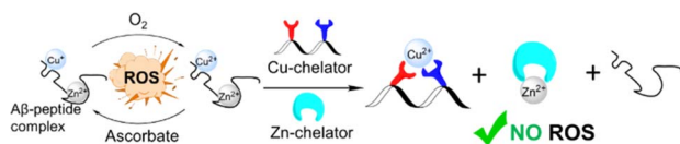
Scheme 1 Schematic representation of a cocktail of two structurally different peptoid-based chelators, designed to selectively bind Cu and Zn ions from the A \beta -peptide complex, stopping the production of ROS in the context of AD.
