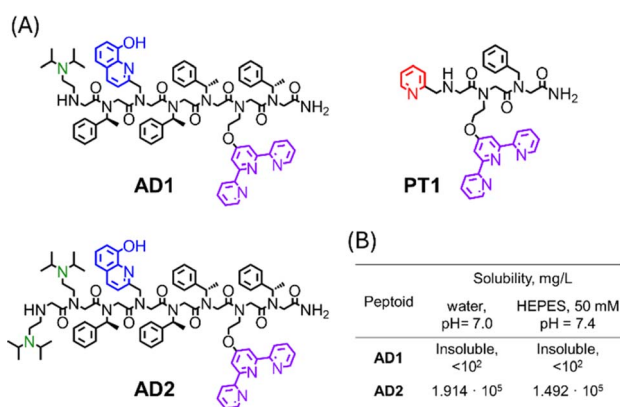
Fig. 1 (A) Chemical structures of peptoid oligomers AD1 – AD2 and PT1 . (B) Solubilities of peptoid AD1 and AD2 in un-buffered water (pH = 7.0) and HEPES buffer (50 mM, pH = 7.4).
