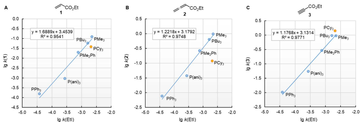
Fig. 7 Reactivities ( \lg k_2 ) of \text{PR}_3 towards (A) ethyl acrylate (1), (B) ethyl allenolate (2), and (C) ethyl propiolate (3) correlate linearly with the S_{\text{N}}2 reactivity of \text{PR}_3 towards ethyl iodide (in acetone at 35 °C, ref. 29b). With rate constants k_2 from Table 3, data for the sterically encumbered \text{PCy}_3 excluded when constructing the correlation lines.
