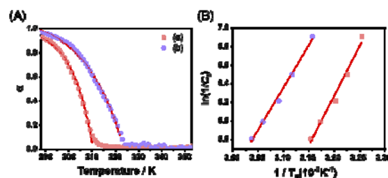
Fig. 7 (A) Degree of aggregation ( \alpha ) in different concentrations of Pt-L 1 (2.0 mM) with 1.5 equiv. of (a) AgNO 3 and (b) Fe(BF 4 ) 2 as a function of temperature at 620 and 650 nm in DMSO/H 2 O (9 : 1 v/v). (B) Natural logarithm of the reciprocal C T as a function of the reciprocal T e showing the linear relationship.
