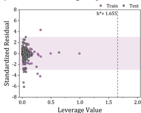
Fig. 12 Applicability domain assessment using William plots: (A) electrical conductivity, (B) ammonia sensing response, (C) toluene sensing response, and (D) benzene sensing response models.
