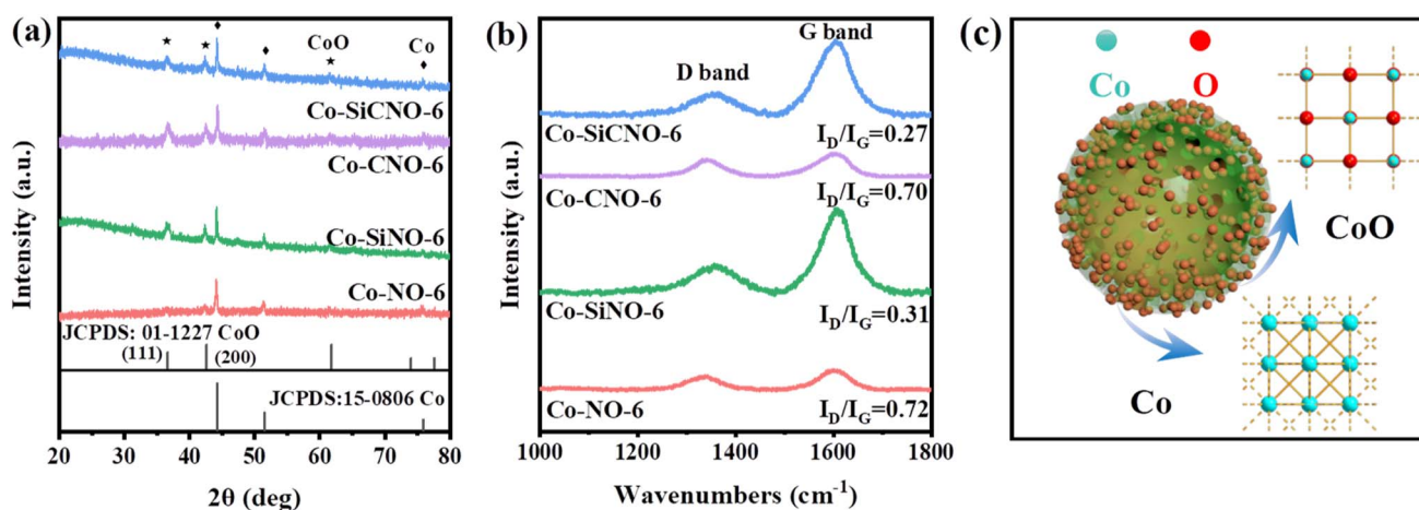
Fig. 2 (a) Wide-angle XRD patterns and (b) Raman spectra of Co-SiCNO-6, Co-CNO-6, Co-SiNO-6 and Co-NO-6; (c) crystal cell structure of multiple Co species in the catalyst.
