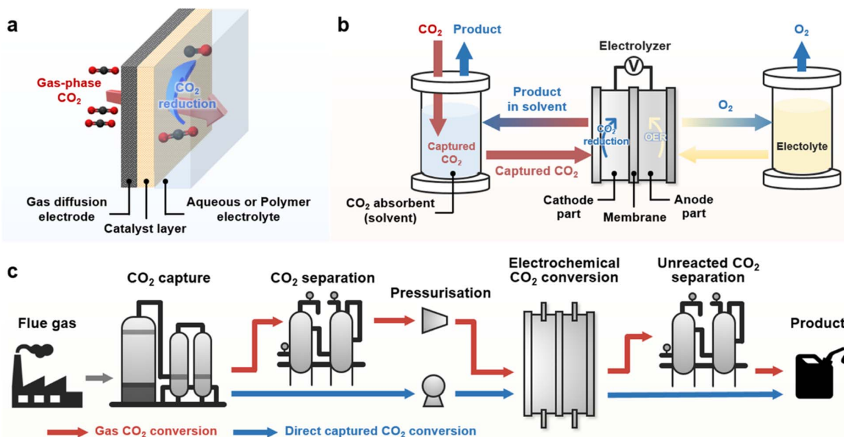
Fig. 1 (a) Schematic of the GDE electrolyser for e\text{CO}_2\text{R} . (b) System for capt- e\text{CO}_2\text{R} . (c) Comparison of the systematic pathway of conventional gas- e\text{CO}_2\text{R} (red line) and capt- e\text{CO}_2\text{R} (blue line).
