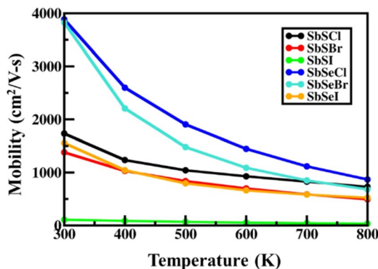
Fig. 4 Carrier mobility of 2D Janus SbYZ monolayers.
