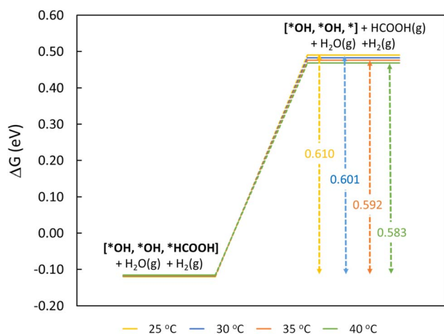
Fig. 9 Free energy diagram for rate-limiting step of \text{HCOOH} desorption as a function of temperature on the 2\text{Ni@SnO}_2(110) model.
