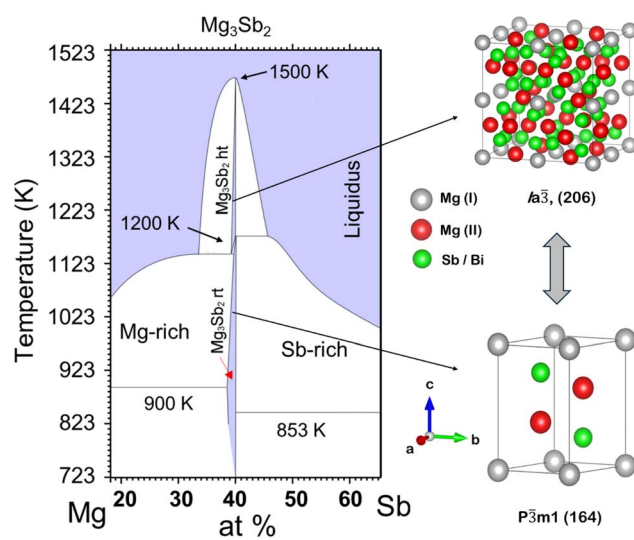
Fig. 1 The Mg–Sb phase diagram near \text{Mg}_3\text{Sb}_2 indicating the phase transformation of \alpha - \text{Mg}_3\text{Sb}_2 ( P\bar{3}m1, 164 ) \leftrightarrow \beta - \text{Mg}_3\text{Sb}_2 ( \text{Ia}\bar{3}, 206 ). 16-18
