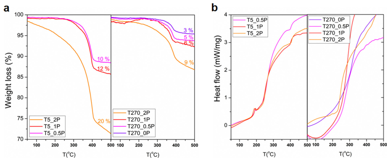
Fig. 5 (a) Thermogravimetric analysis of the synthesized samples of Bi 19 S 27 I 3 at different reaction times and PEG:Bi molar ratios. (b) Differential scanning calorimetry of the synthesized samples of Bi 19 S 27 I 3 at different reaction times and PEG:Bi molar ratios.
