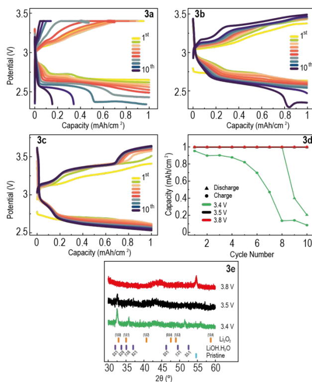
Figure 3 Constant Current Constant Voltage protocol with redox mediator. a-c) CCCV potential curves of \text{Li-O}_2 cells containing LiI as a redox mediator in the electrolyte cycled at a range of upper-cut-off voltages (UCVs); a) 3.4 V, b) 3.5 V and c) 3.8 V. d) Discharge and charge capacity per cycle. e) XRD patterns of electrodes taken after the 10th discharge-charge cycles.
