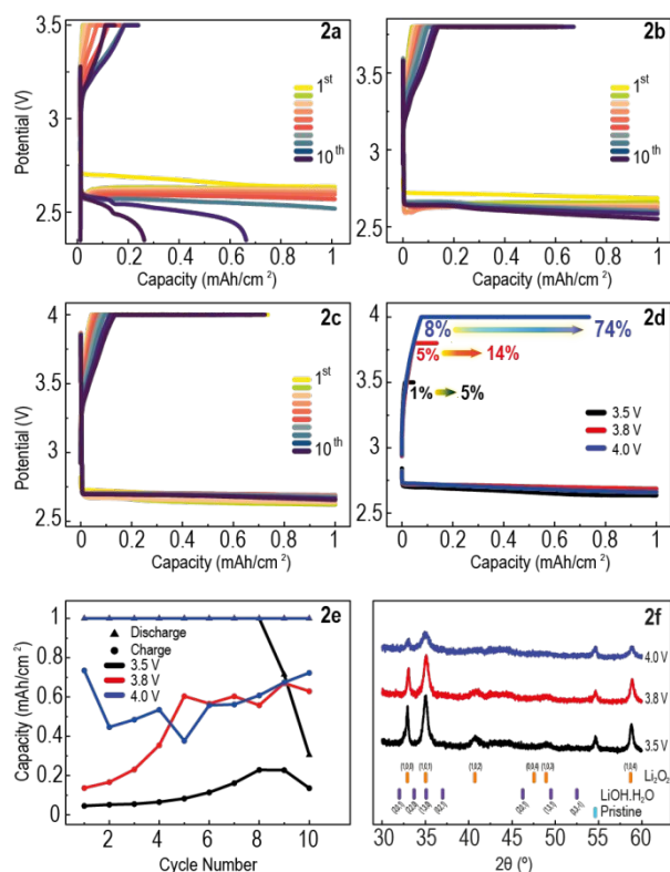
Figure 2 Constant Current Constant Voltage protocol. a-c) CCCV potential curves of \text{Li-O}_2 cells cycled at a range of upper-cut-off voltages (UCVs); a) 3.5 V, b) 3.8 V and c) 4.0 V. d) CCCV potential curves of the first discharge-charge cycle of \text{Li-O}_2 cells showing capacity recovered during the CC portion of charge and subsequent capacity recovered during the CV portion of charge. e) Discharge and charge capacity per cycle comparison. f) XRD patterns of electrodes taken after the 10th discharge-charge cycles.
