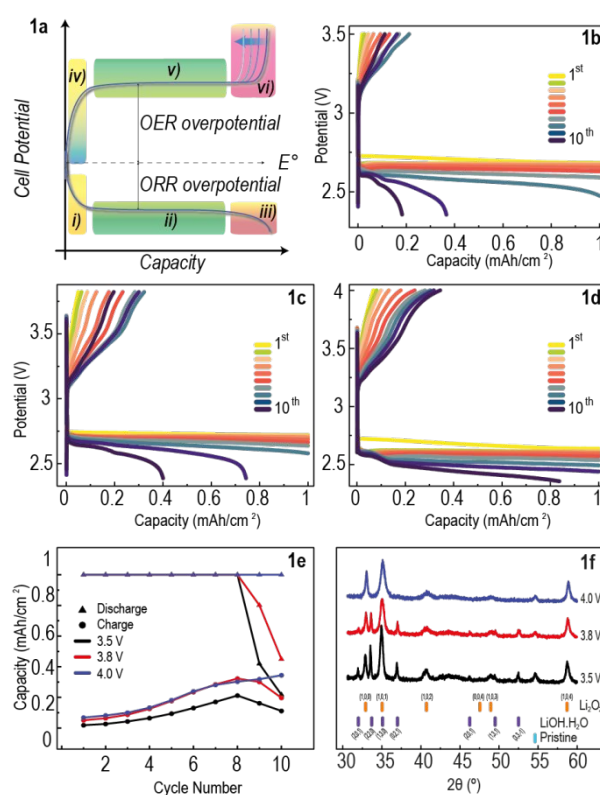
Figure 1 Constant Current protocol. a) Typical galvanostatic cycling (CC) potential curves of Li-O 2 cells. b-d) CC potential curves of Li-O 2 cells cycled at a range of upper-cut-off voltages (UCVs); b) 3.5 V, c) 3.8 V, and d) 4.0 V. e) Discharge and charge capacity per cycle comparison. f) XRD patterns of electrodes taken after the 10th discharge-charge cycles.
