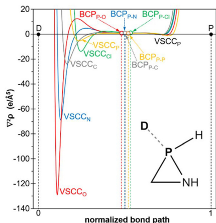
Fig. 10 Computed (B3LYP/def2-TZVPP//B3LYP-D4/def2-TZVPP) variation of the Laplacian of the electron density at the central part of the donor-phosphorus normalized bond path in encounter complexes 1a -(nucleophile), for Cl - (green), MeOH (red), MeNH 2 (blue), NHC Me2 (grey) and PMe 3 (orange).
