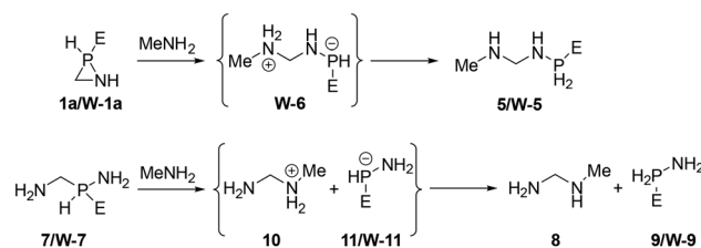
Scheme 3 Methyl amine-mediated P–C bond cleavage in parent ( 1a ) and W(CO) 5 complexed ( W-1a ) azaphosphiridine and model acyclic analogues 7 and W-7 .
