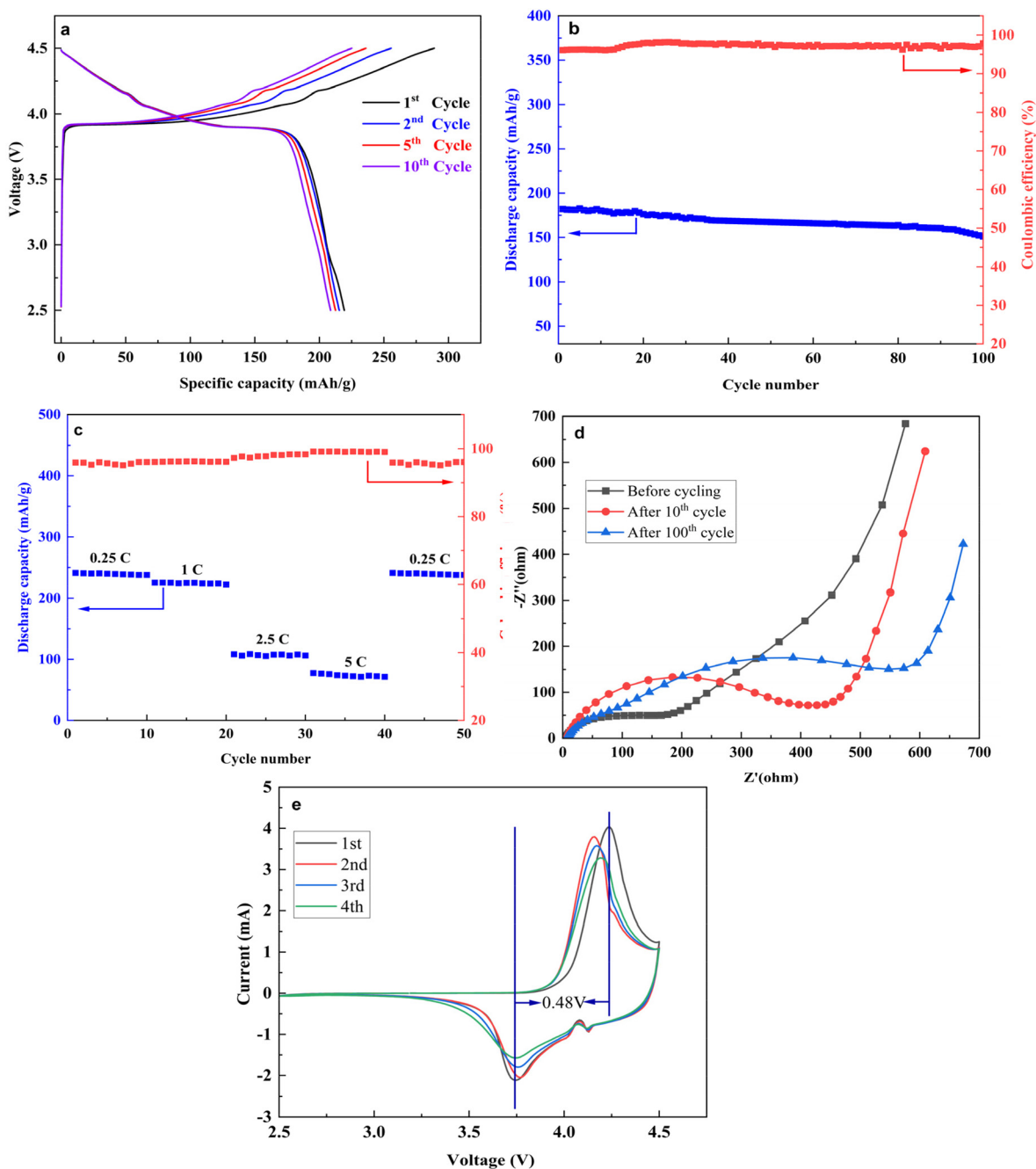
Fig. 10 (a) Charge–discharge curve; (b) cycle performance of the generated \text{LiCoO}_2 ; (c) rate performance; (d) EIS spectra; (e) CV curve of regenerated \text{LiCoO}_2 .
